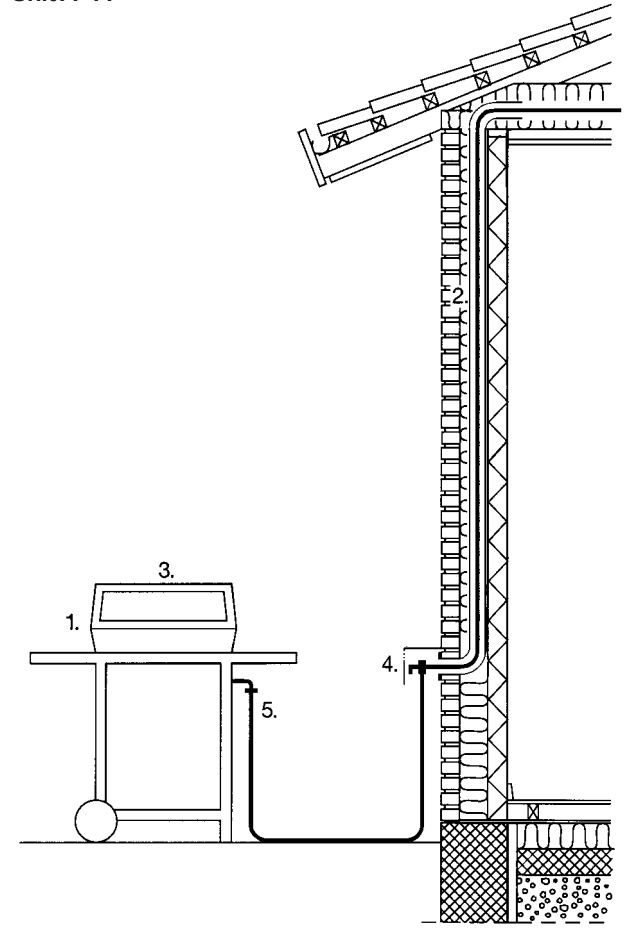
Snit A - A
